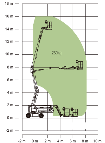
Range of Motion ZA14NJE/ZA14NJE-Li
